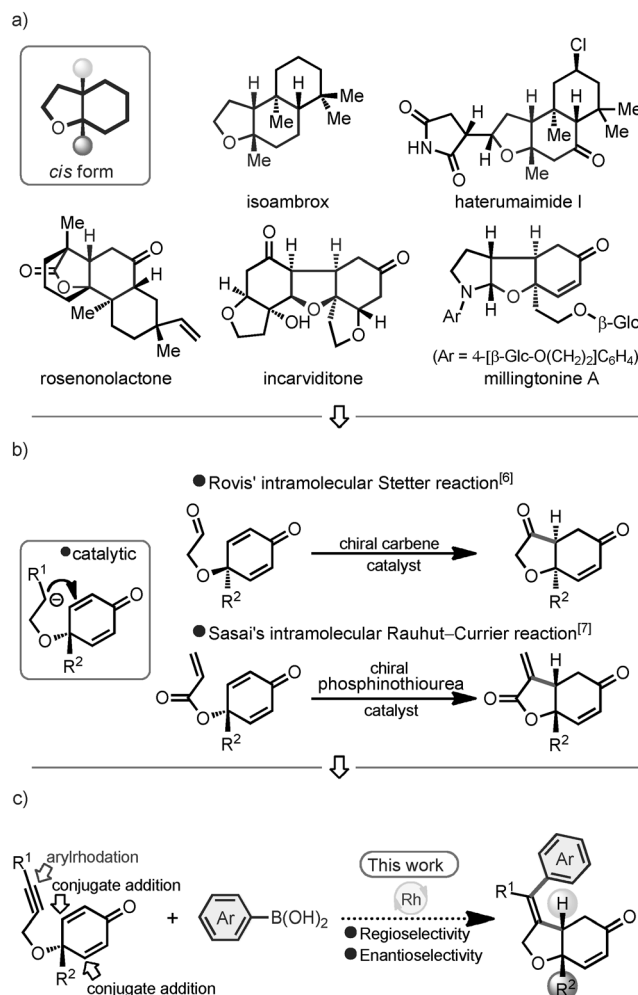
Scheme 1. Catalytic asymmetric desymmetrization of cyclohexadienones for preparing chiral cis -hydrobenzofurans. a) cis -Hydrobenzofurans as structural motifs in natural products. b) Organocatalytic asymmetric desymmetrization of cyclohexadienones. c) Our approach to enantioenriched cis -hydrobenzofurans.
