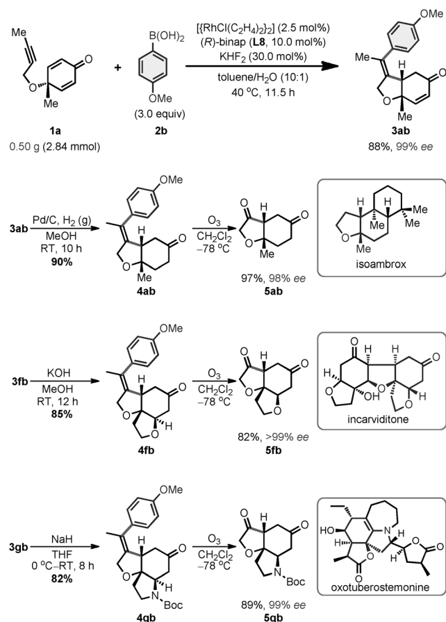
Scheme 4. Half-gram scale reaction and transformations of the cyclization products. THF = tetrahydrofuran.
