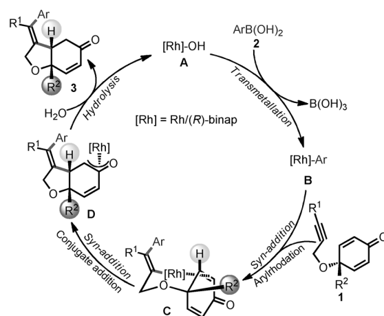
Scheme 3. Proposed mechanism for this tandem reaction.
