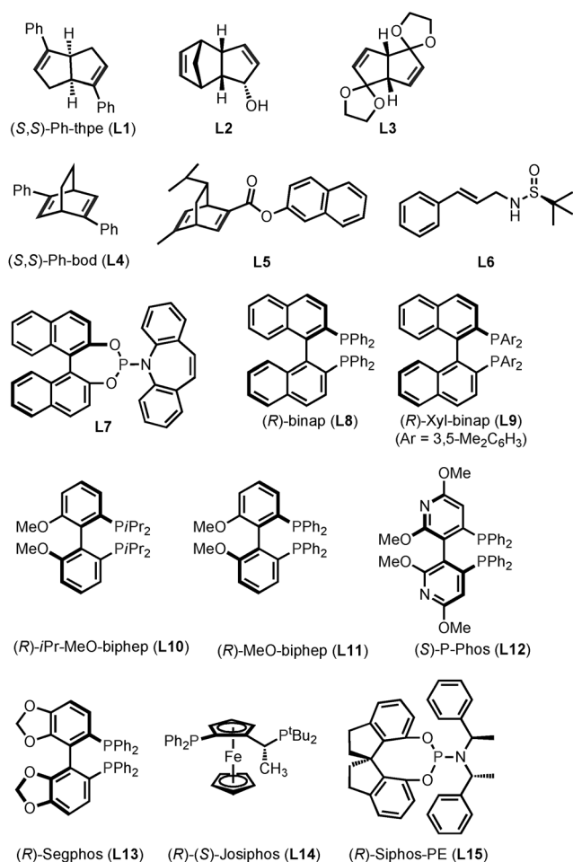
Scheme 2. Structures of chiral ligands.
